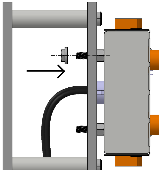
Fig. 4.33: Insert the M5 flange nuts onto the screw
