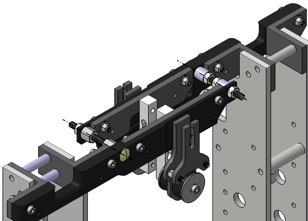
Fig. 4.47: Cut view of two bolts connecting two load measurement units (using two methods)
