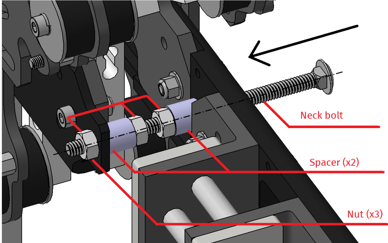
Fig. 4.46: Bonding two load measurement units with neck bolt, spacers and nuts (Possible action 2)
