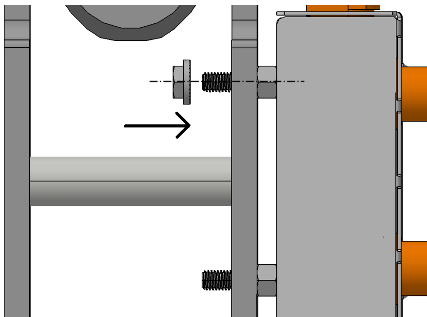
Fig. 4.29: Insert the nuts to fix the no-solder board onto the support plate
