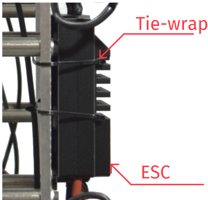
Fig. 4.30: Example on fixing ESC on the support plate using tie-wraps
