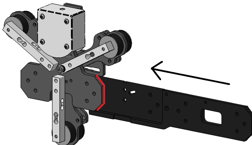
Fig. 4.41: Slide the special mount plate into the load measurement unit using highlighted feature
