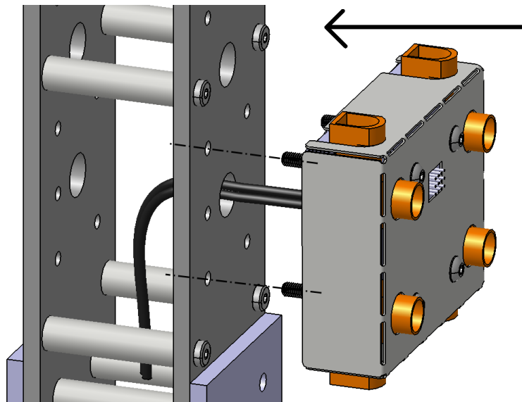
Fig. 4.32: Insert the power and control console onto the support plate
