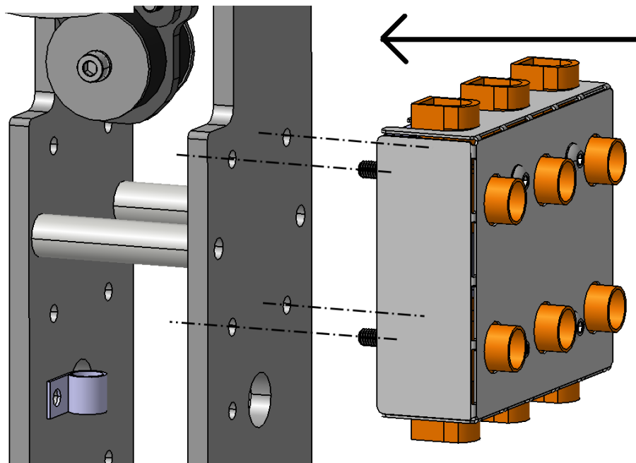
Fig 4.28: Insert the no-solder board on the support plate
