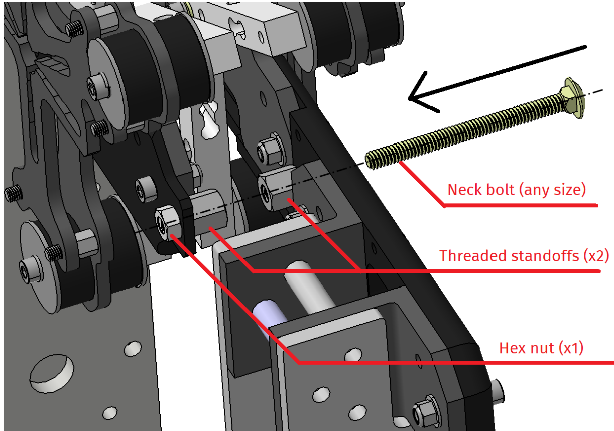
Fig. 4.45: Bonding two load measurement units with neck bolts and standoffs (Possible action 1)
