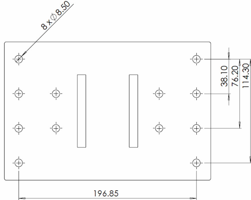
Fig. 3.2: Fixture base plate (#KGTP): adapter to place and hold the S1780 on the rails. This part comes with the railing system accessory, or can be purchased separately.
