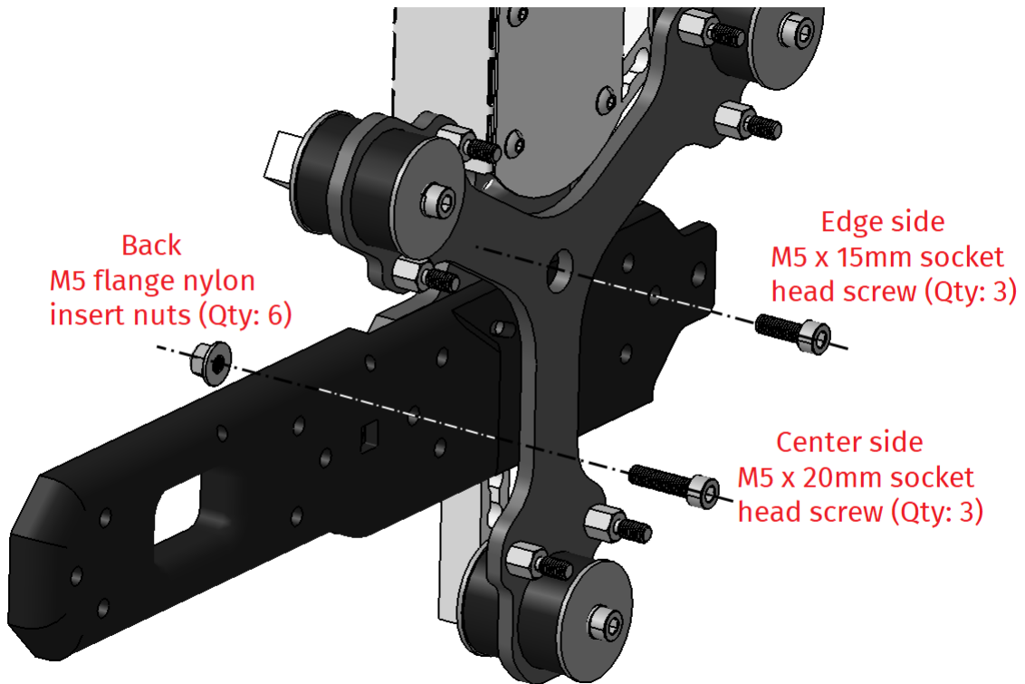
Fig. 4.43: Fasteners to tighten the special mount and the load measurement unit
