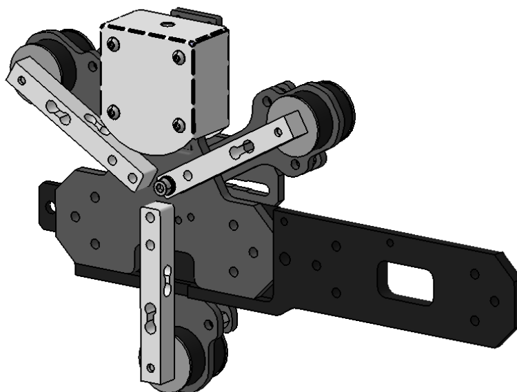
Fig. 4.42: The coaxial back-to-back special mount completely inserted into the load measurement unit
