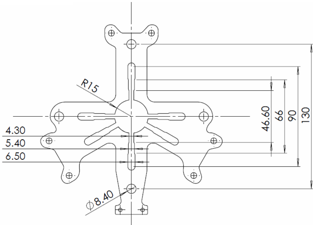
Fig 4.21: XLCH motor mount with D=30 mm center hole
