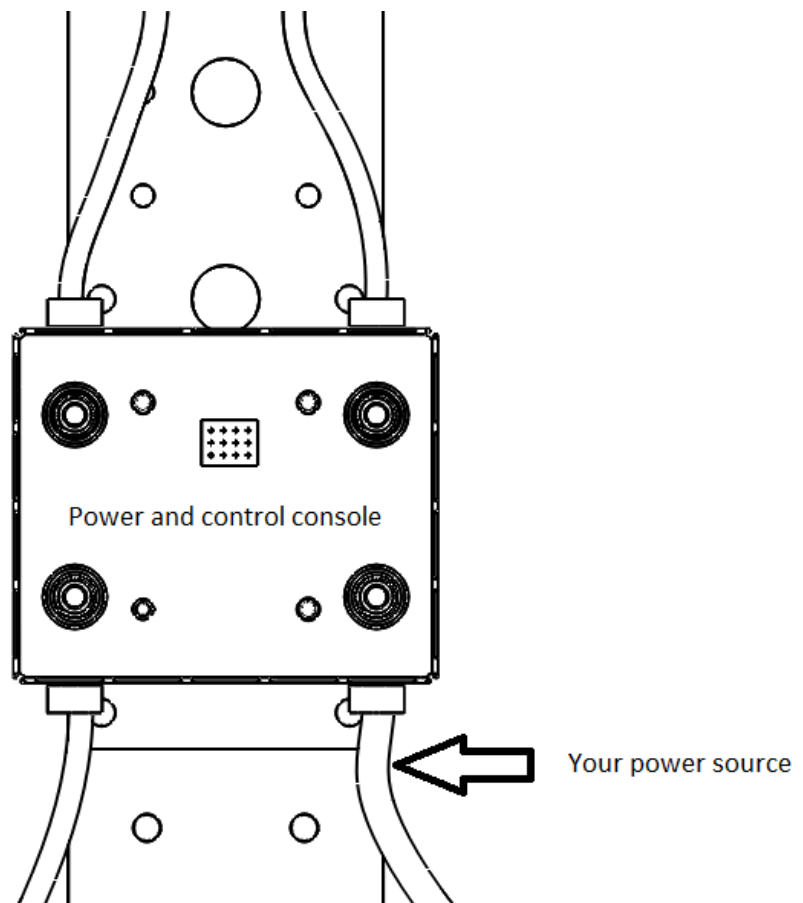
Fig. 5.3: Power chain between power and control console and your power source
