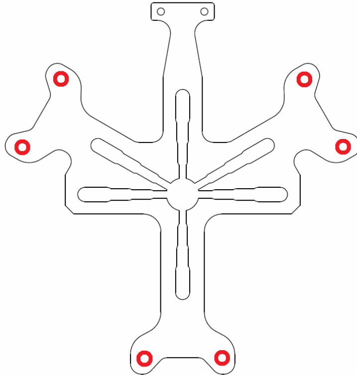
Fig. 4.25: Use the highlighted 6 holes feature to align with the load measurement unit
