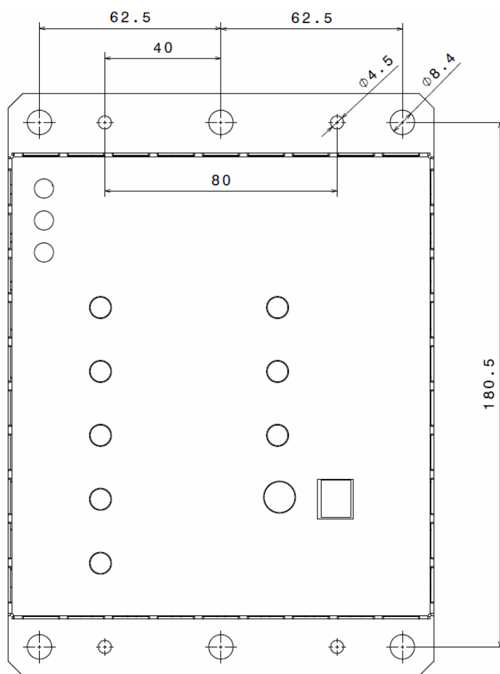
Fig. 4.35: Schematic drawing for main board mounting holes
