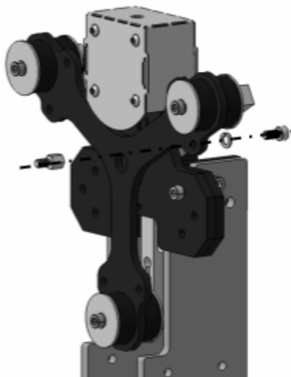
Fig. 4.24: Connection of the screw, washer and the standoff to the load measurement unit
