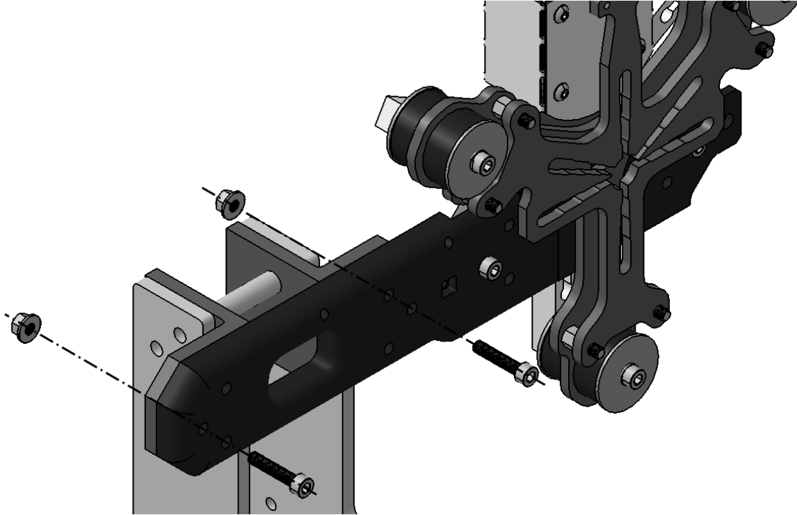
Fig. 4.44: Insertion of fasteners to connect the special mount and the two-plate support
