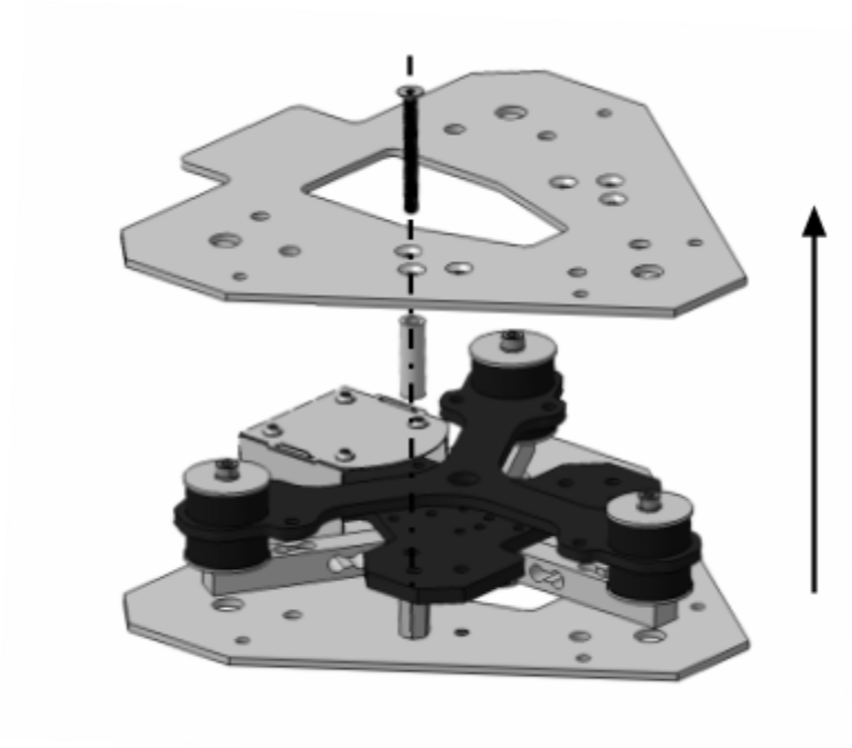
Fig. 4.16: Removal of the protective metal plate
