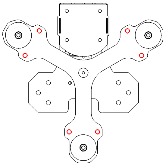
Fig. 4.23: Use the highlighted 6 holes feature to place your screws and split lock washers
