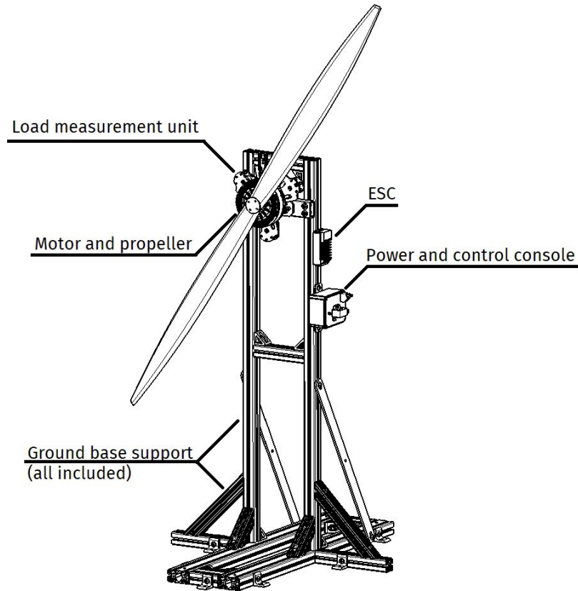
Fig. 2: Hardware overview for 75kgf version
