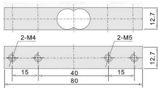
Fig. 5: General dimensions of the load cell
