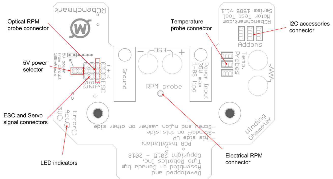
Fig 6: Top layout
