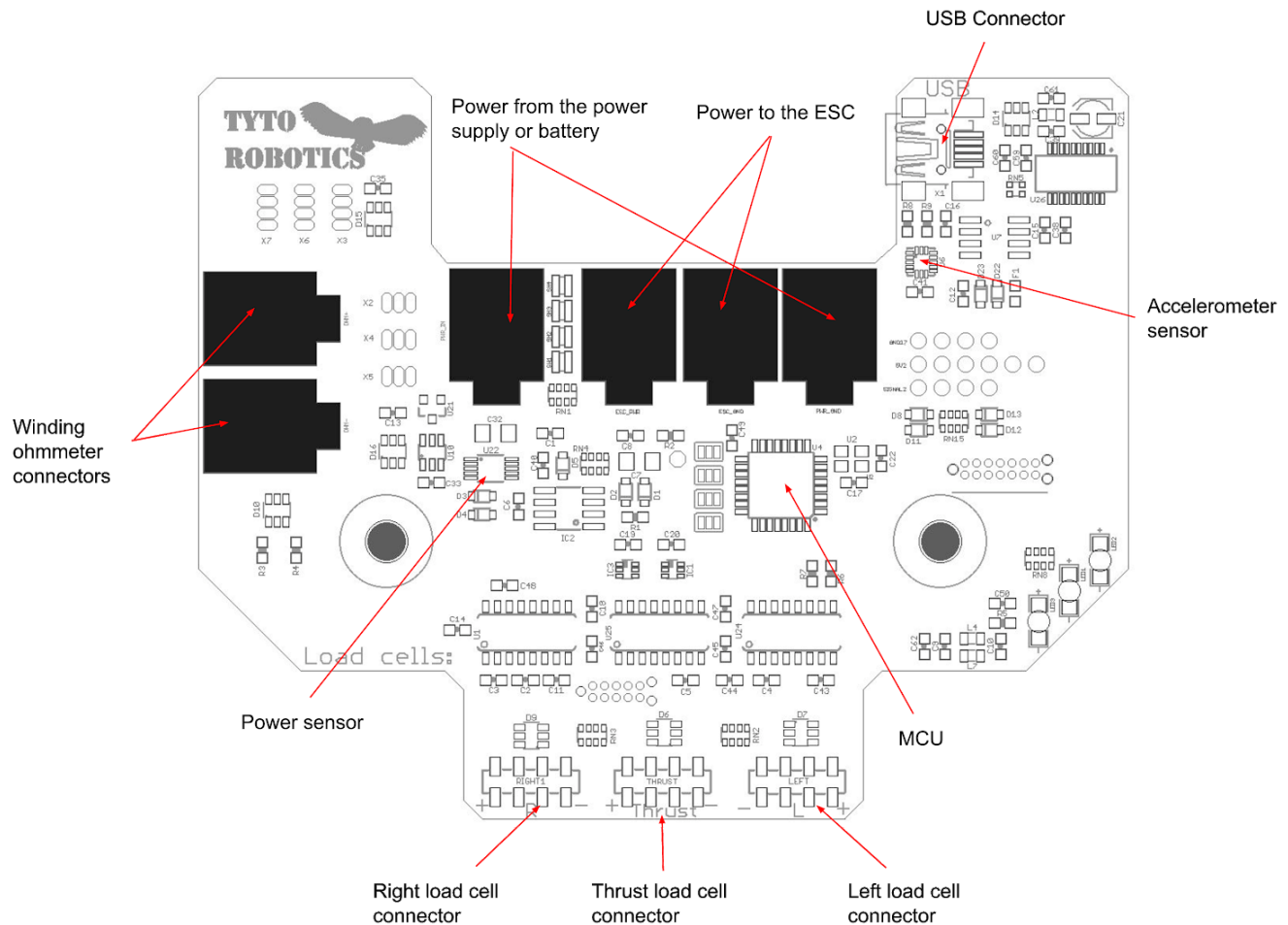
Fig 7: Bottom layout
